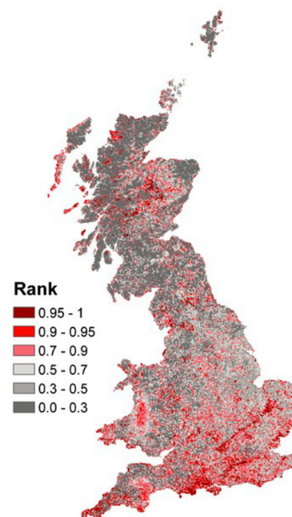
Option 3. Priority regions for biodiversity only
