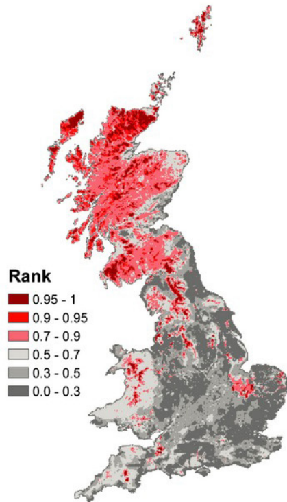
Option 1. Priority regions for carbon restoration only
