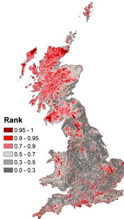
Option 2. Priority regions for both carbon and biodiversity
