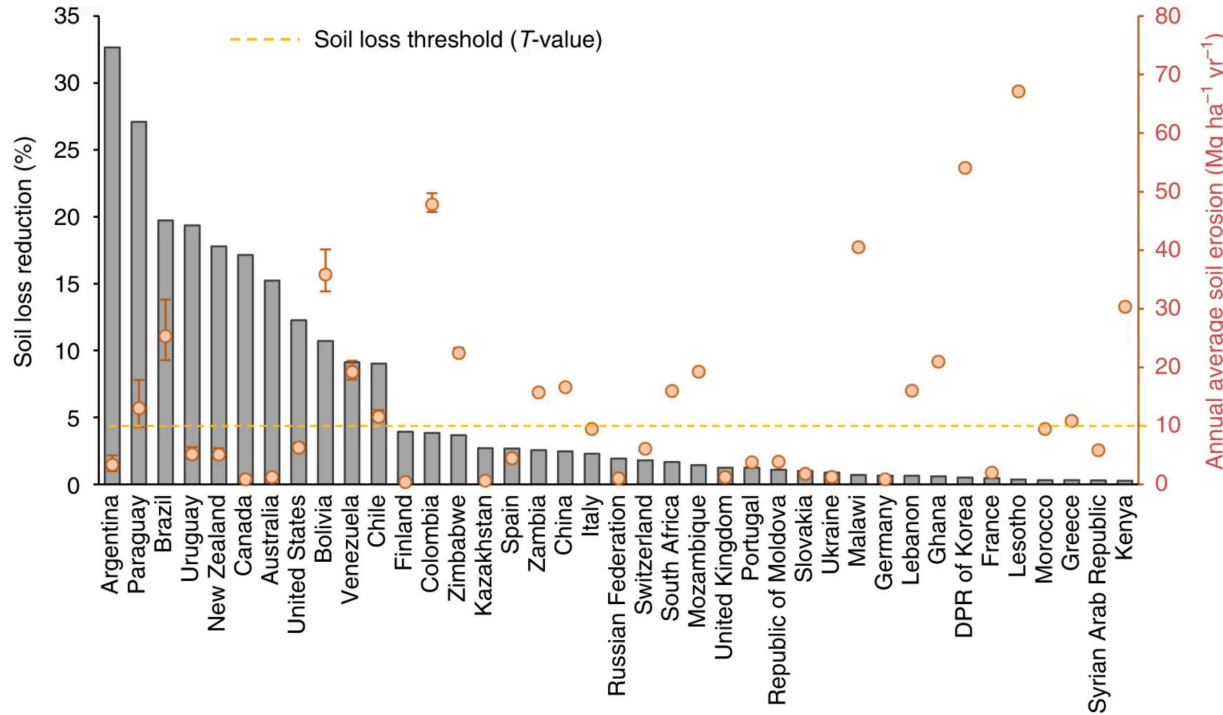
Chart shows (grey bars) reductions in soil loss associated with adopting conservation agriculture globally, alongside current erosion rates (orange dots). The UK has very low soil erosion (as little UK forest is being converted to cropland), though the analysis only modelled data up to 2012. However, the UK imports food from countries with high soil loss rates.
